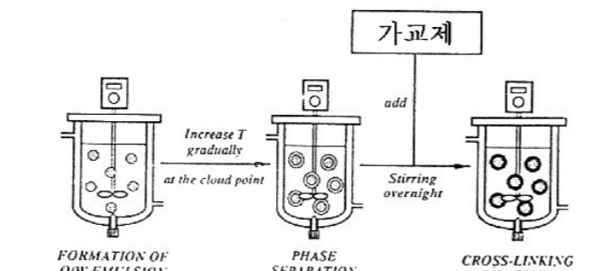
Figure 2. Schematic microcapsule by coacervation method
