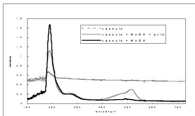
Figure 7. Spectra of cross-linked PVA
