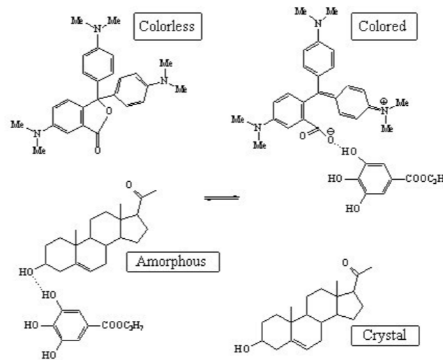
Figure 3. Schematic explanation of rewritable mechanism
