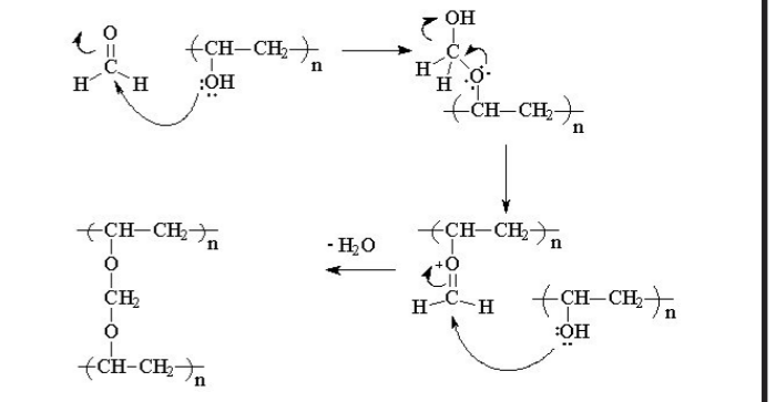
Figure 5. Cross-linking mechanism of PVA
