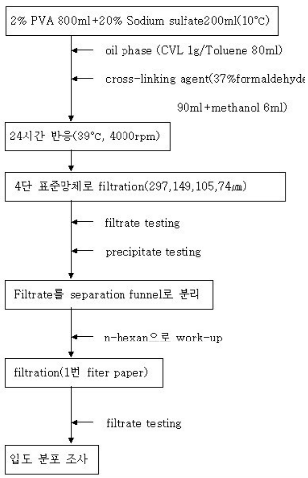
Figure 6. Flow chart for Microencapsulation
