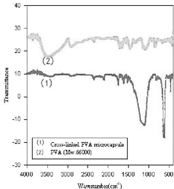
Figure 8. FT-IR spectra of microcapsule
